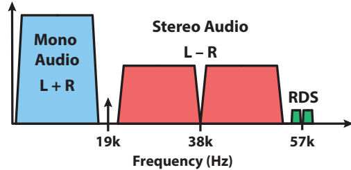
Figure 3: Structure of FM Radio Transmissions. Baseband audio signals transmitted in stereo FM broadcasts.
