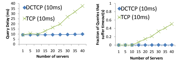
Figure 19: Many-to-one: With dynamic buffering, DCTCP does not suffer problems at even high load.
