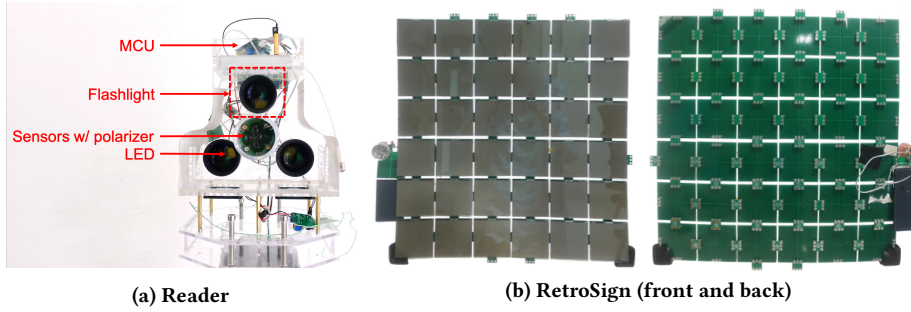
Figure 8: Retrol2V prototype.
