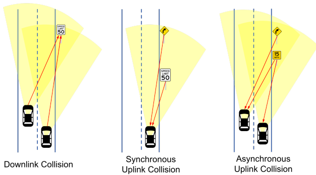
Figure 4: Illustration of different collision scenarios.
