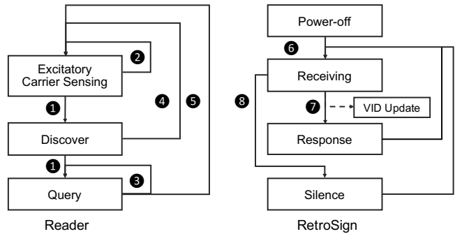
Figure 5: States and transitions in RetroI2V end devices: 1 One-to-one communication, the normal communication case. 2 Overhear other ongoing session. 3 Loop over multiple RetroSigns. 4 Downlink collision or no RetroSign in view. 5 Communication ended or aborted. 6 Powered on (by incoming light). 7 On-target communication. 8 Downlink collision or off-target suppression.
